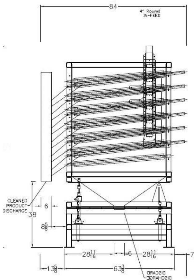
Q-SAGE SBS-6 Soybean Belt Sorter Left Hand (LH) Machine Shown END VIEW (Charge End)
